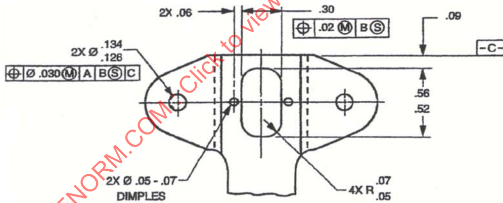
FIGURE 3 - VIEW L-L SHOWING SLOT IN BRACKET
