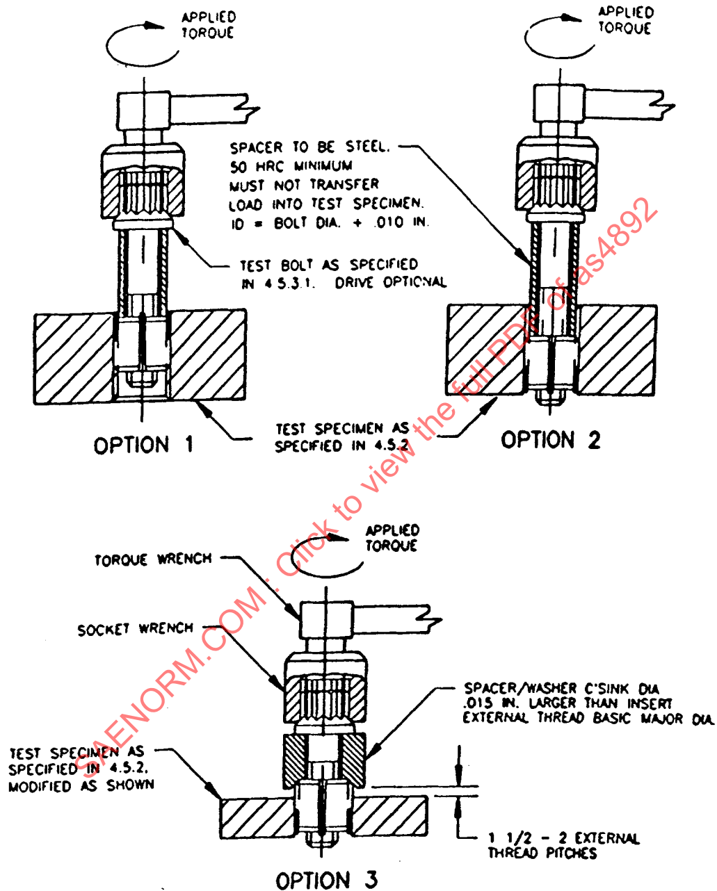
FIGURE 3 - Rotational Resistance Fixture (Options)
