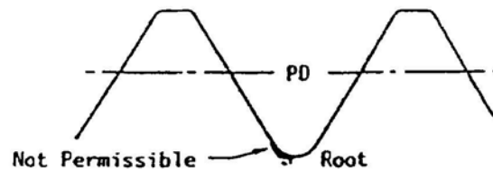
FIGURE 4 - Root Defects, Rolled Thread
