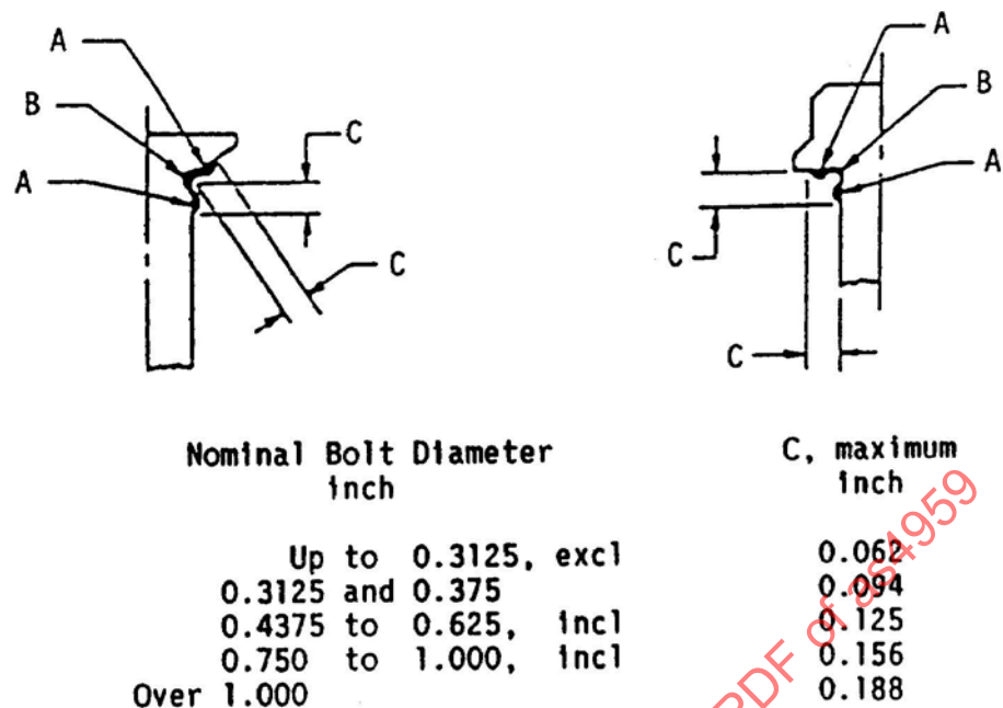
FIGURE 2 - Permissible Distortion From Fillet Working
