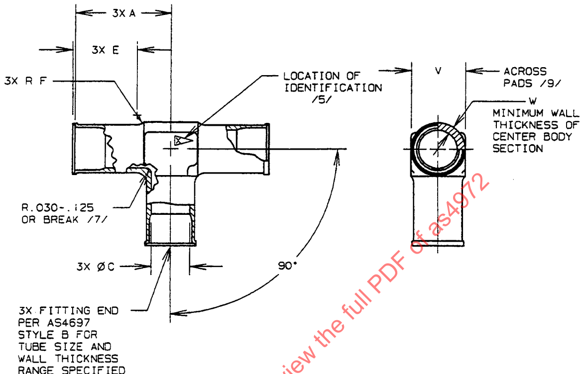
FIGURE 1 - FITTING, TEE
