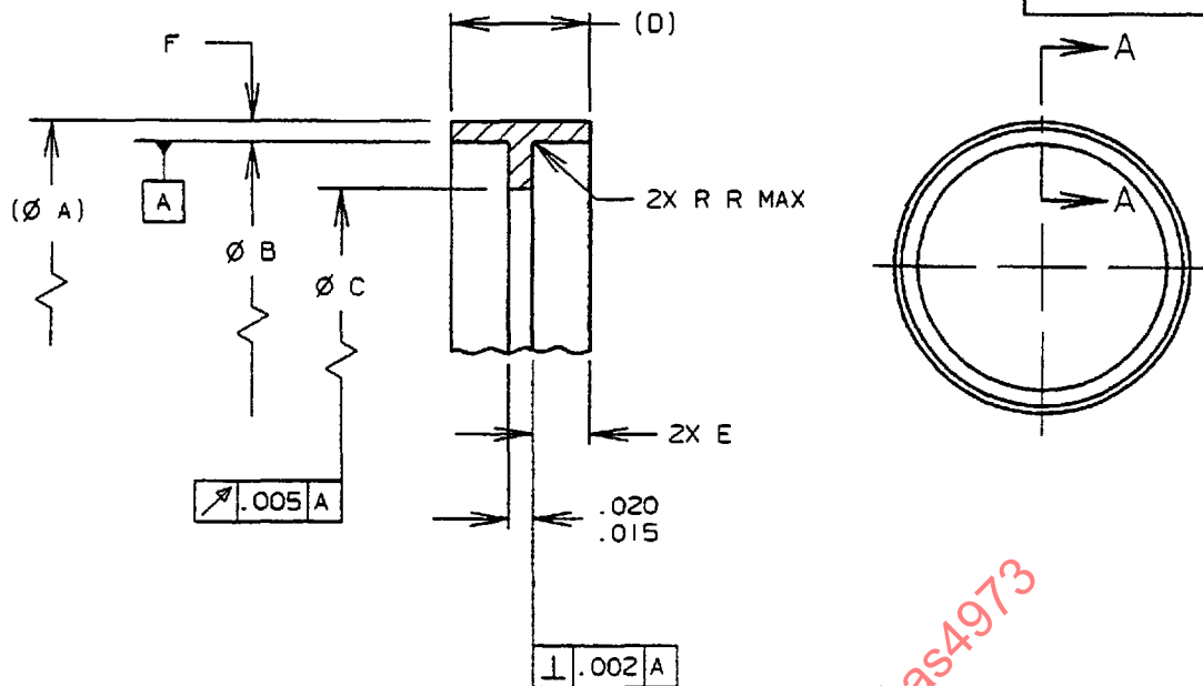
SECTION A-A ENLARGED
