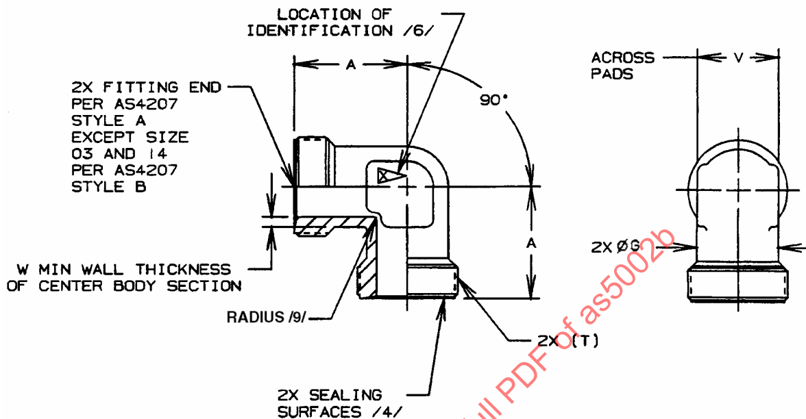
FIGURE 1 - FITTING, ELBOW, 90°
