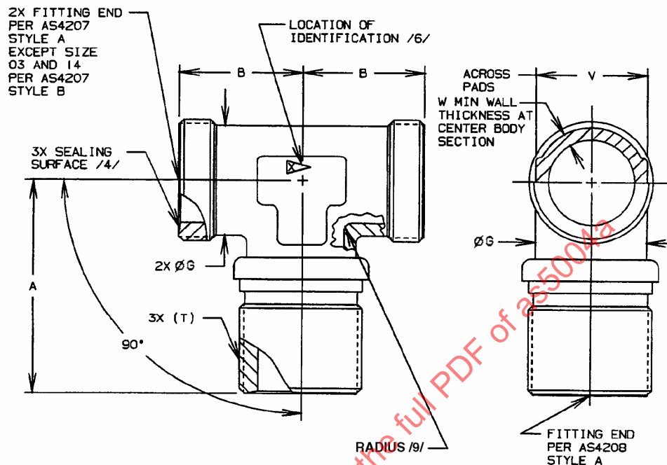
FIGURE 1 - FITTING, TEE, BULKHEAD ON SIDE
