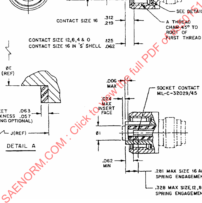
FIGURE 2. Connector, plug, front release, series II, interface dimensions.
