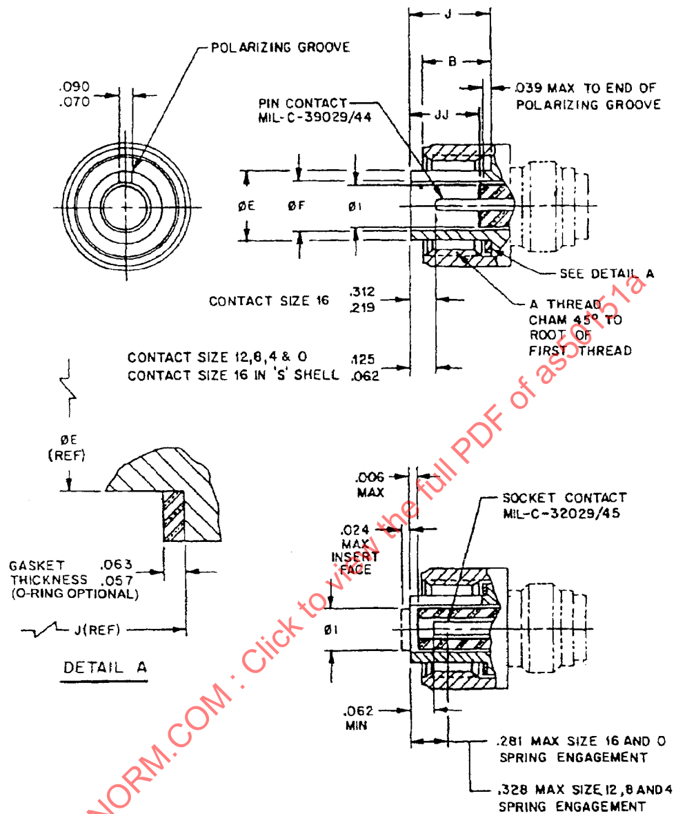
FIGURE 2 - CONNECTOR, PLUG, FRONT RELEASE, SERIES II, INTERFACE DIMENSIONS
