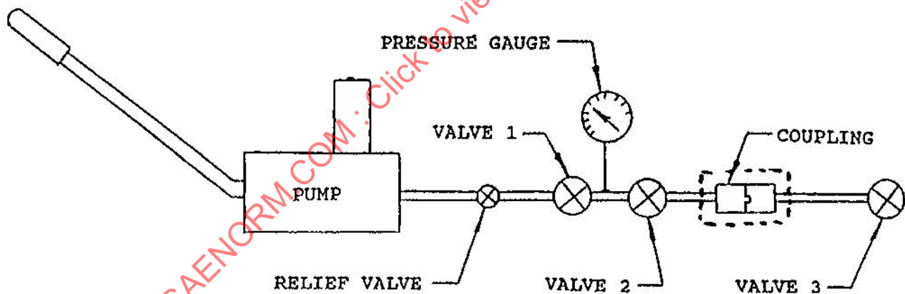
FIGURE 3 - Extreme Temperature Setup
