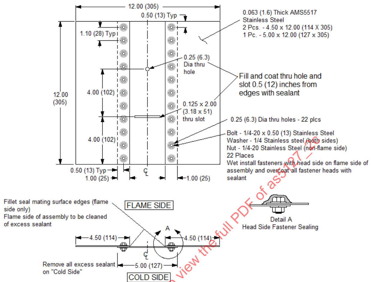
Figure 1 - Sealing assembly
