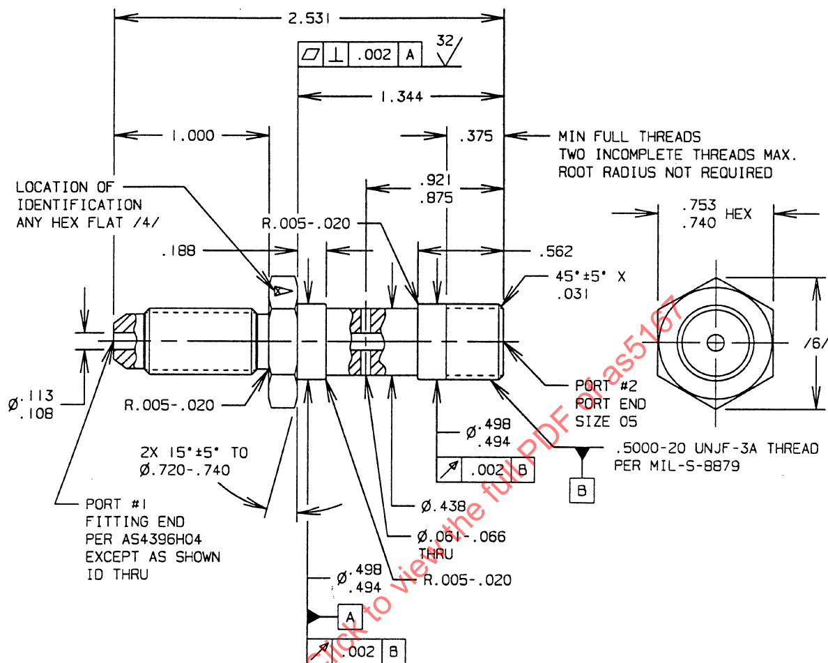
◆ FIGURE 1 - FITTING, ADAPTER
