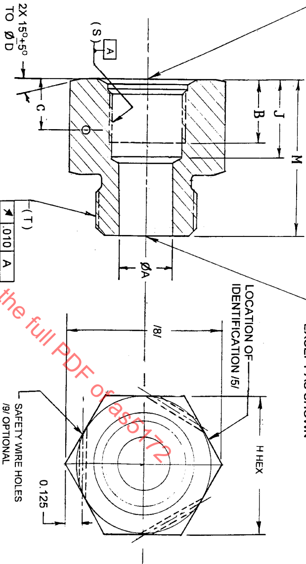
FIGURE 1 - FITTING-ADAPTER
