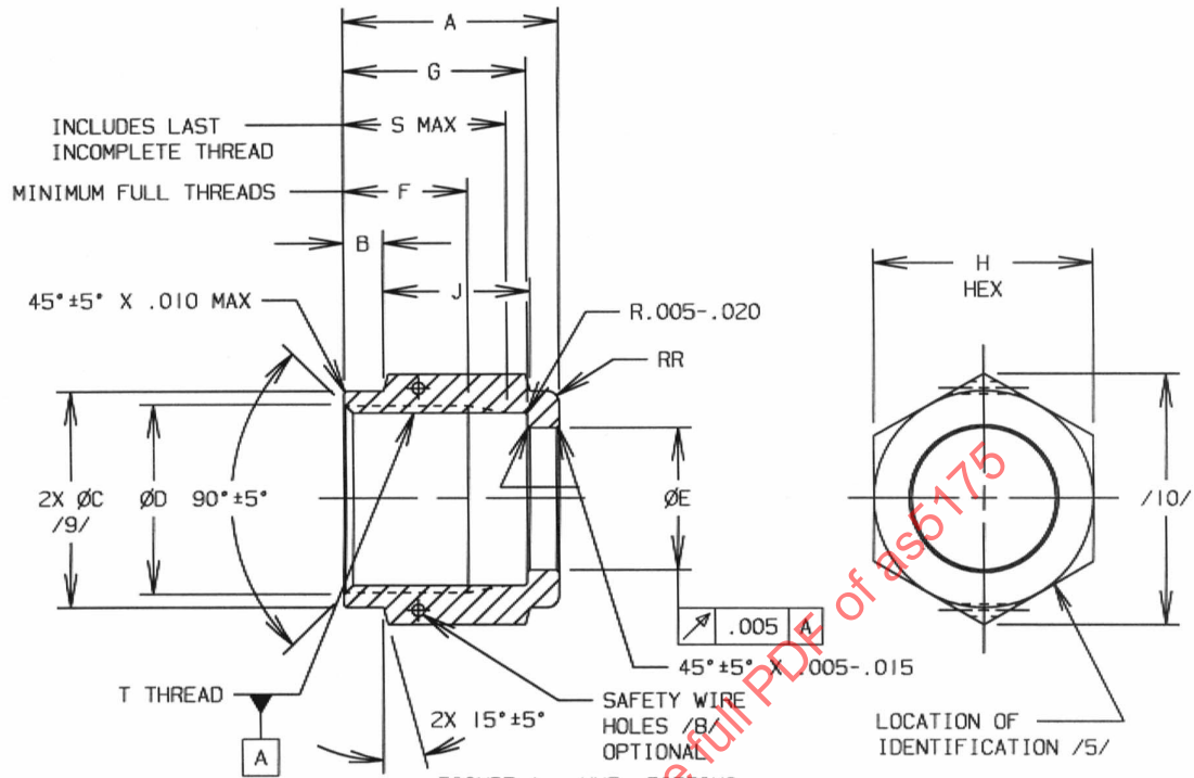
FIGURE 1 - NUT, FITTING
