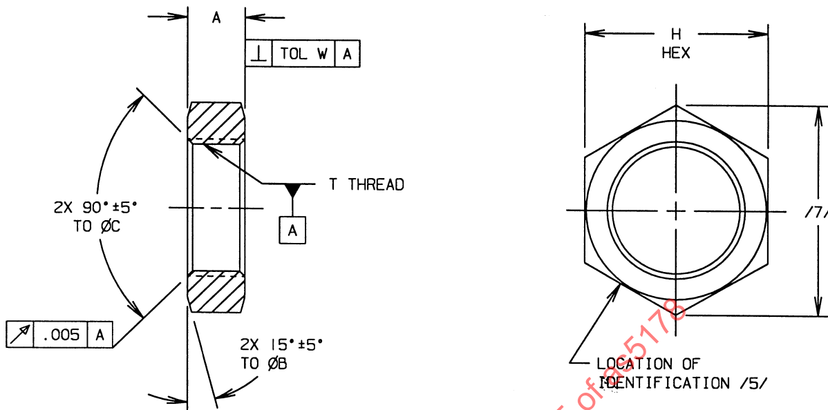
FIGURE 1 - FITTING, NUT
