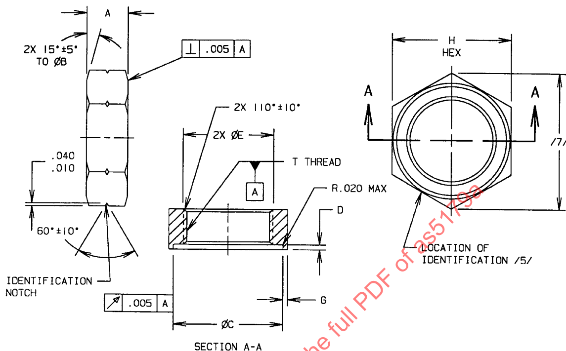
FIGURE 1 - FITTING, NUT
