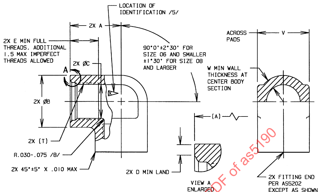
FIGURE 1 - FITTING, ELBOW 90°
