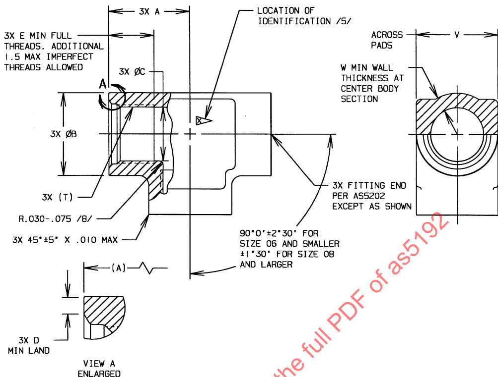
FIGURE 1 - FITTING, TEE
