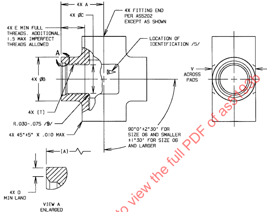
FIGURE 1 - FITTING, CROSS
