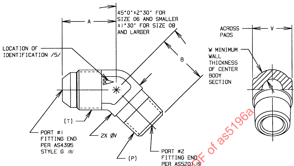
FIGURE 1 - FITTING, ELBOW, 45°
