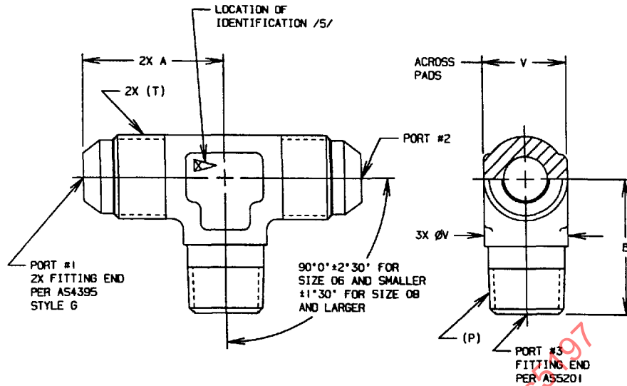
FIGURE 1 - FITTING, TEE
