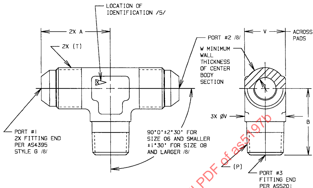
FIGURE 1 - FITTING, TEE
