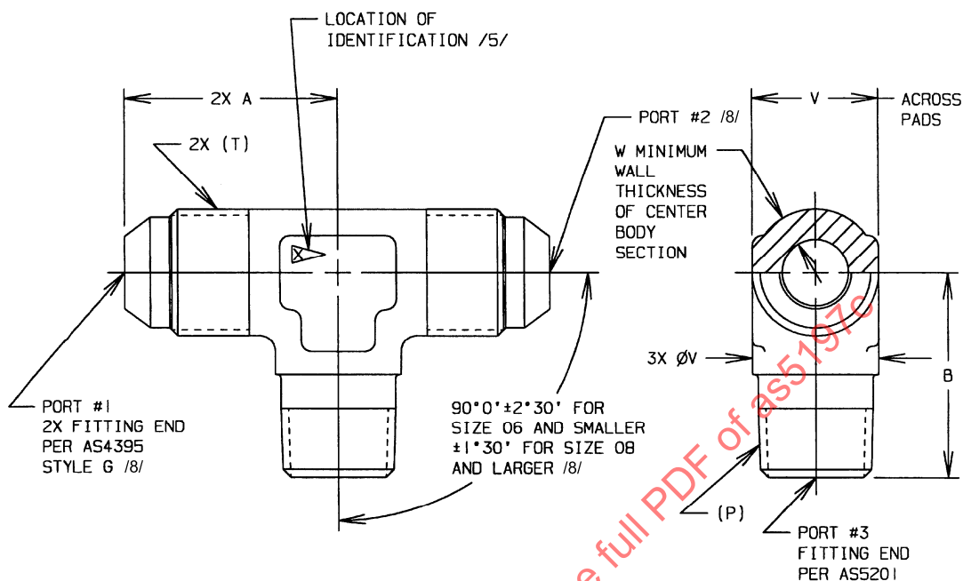
FIGURE 1 - FITTING
