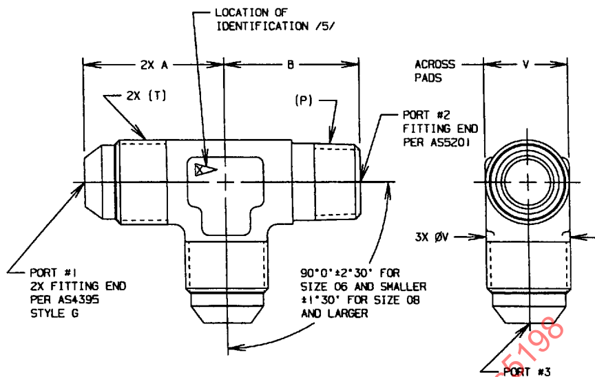
FIGURE 1 - FITTING, TEE
