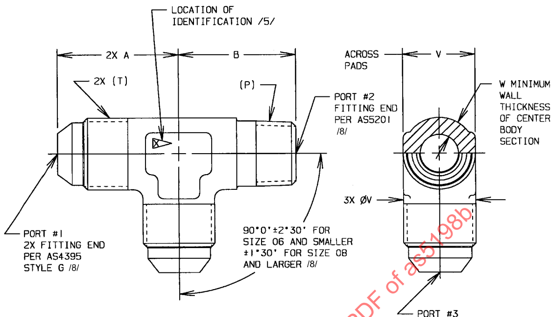
FIGURE 1 - FITTING, TEE
