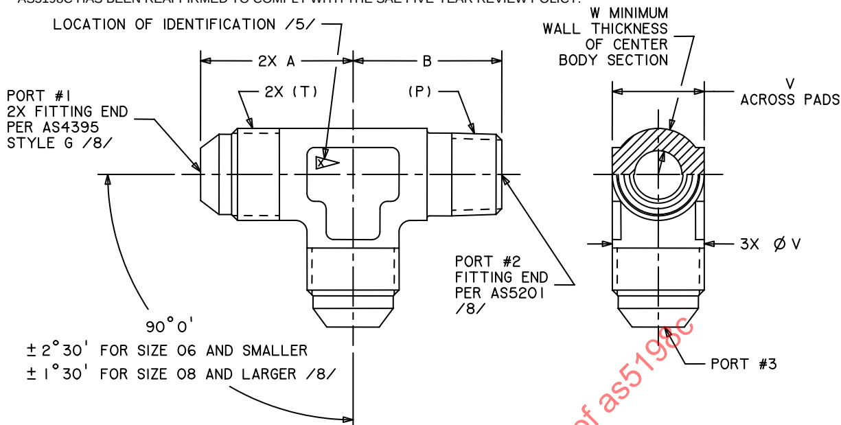
FIGURE 1 – FITTING, TEE TABLE 1 – DIMENSIONS
