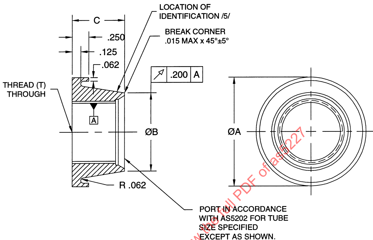
FIGURE 1 - FLANGE
