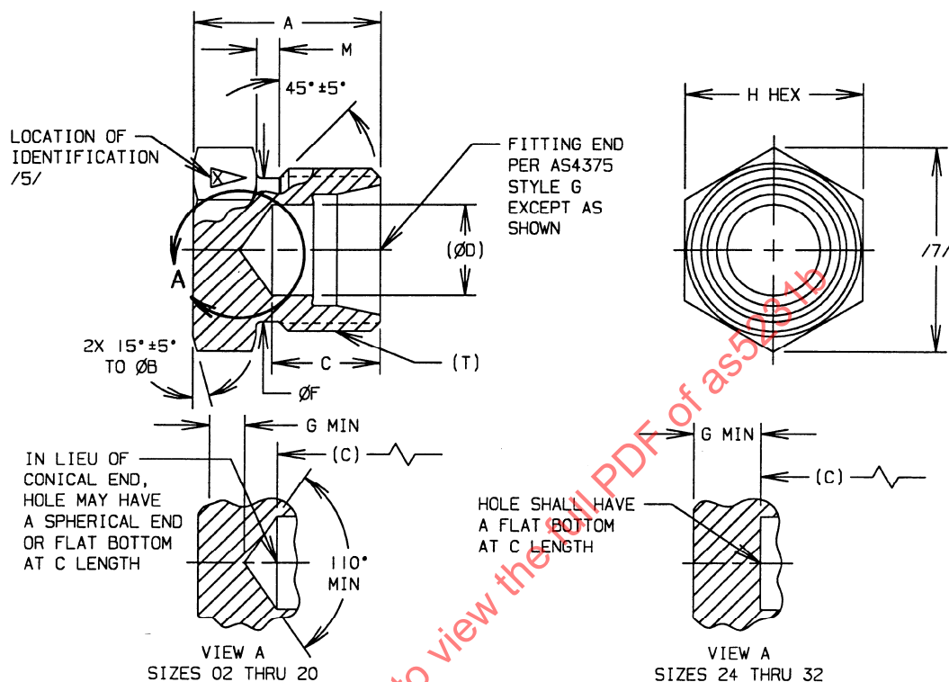
FIGURE 1 - FITTING, PLUG
