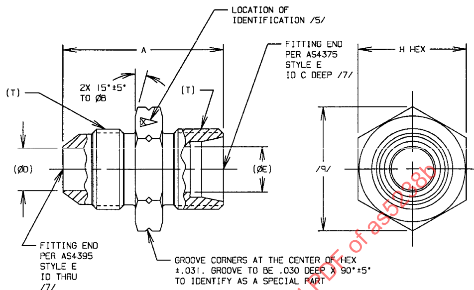
FIGURE 1 - FITTING, ADAPTER
