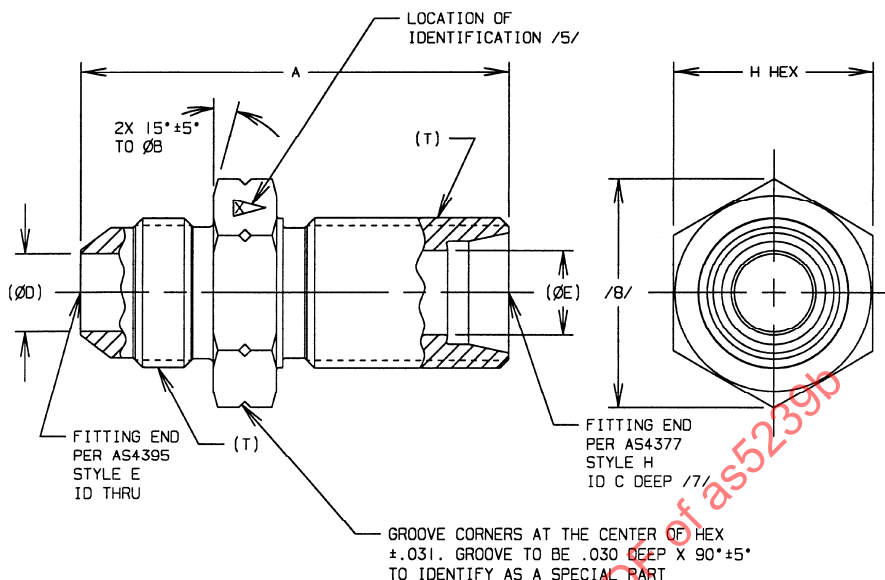
FIGURE 1 - FITTING, ADAPTER
