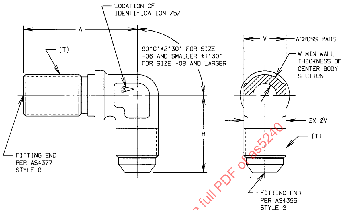
FIGURE 1 - FITTING, ELBOW, 90°
