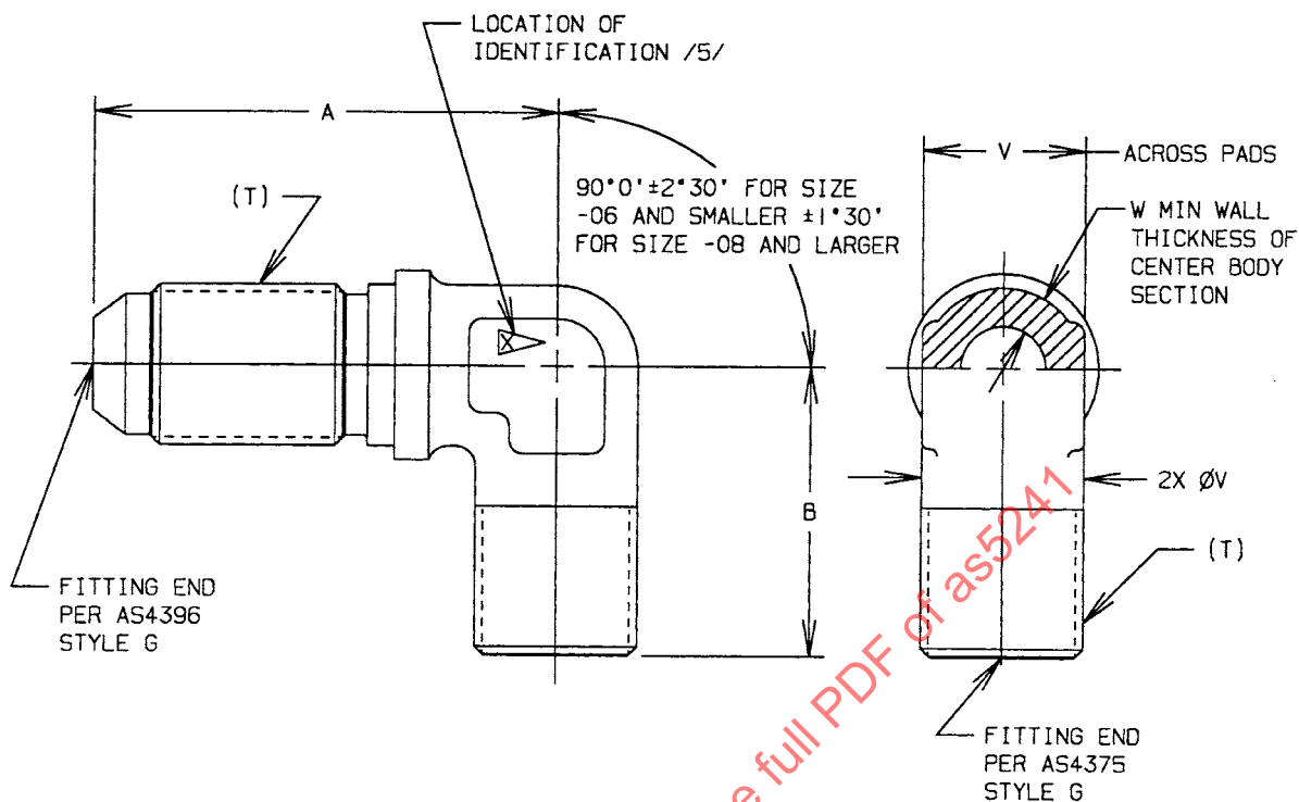
FIGURE 1 - FITTING, ELBOW, 90°
