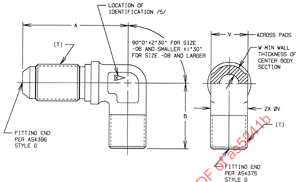
FIGURE 1 - FITTING, ELBOW, 90°
