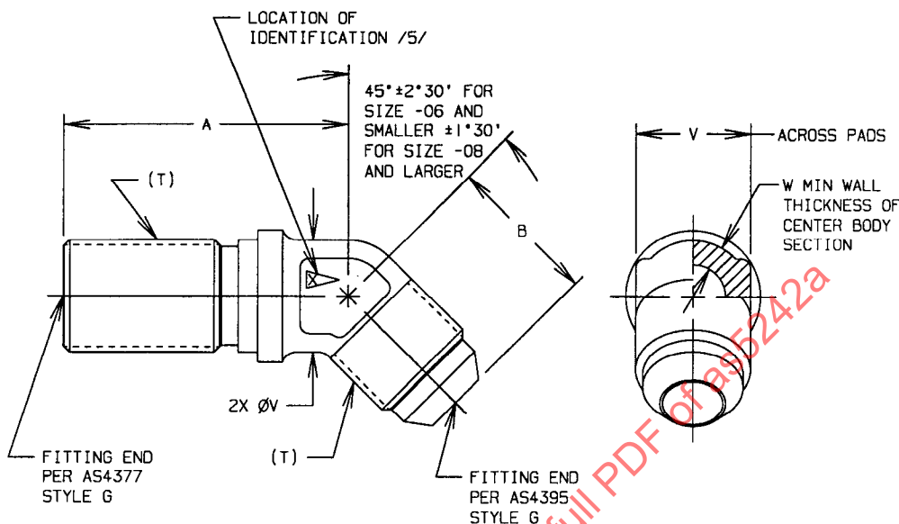
FIGURE 1 - FITTING, ELBOW, 45°
