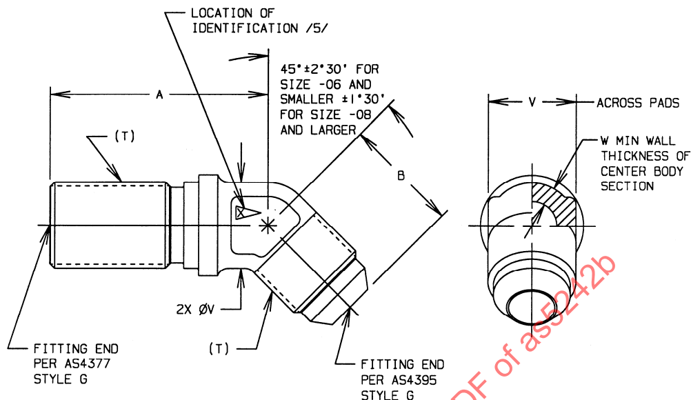
FIGURE 1 - FITTING, ELBOW, 45°
