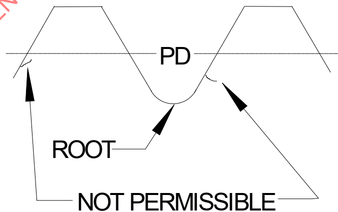
Figure 6 - Lap; below pd in any direction, rolled thread
