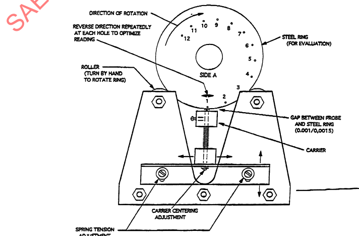
Figure 2 - Schematic of fixture for obtaining manual flux leakage readings
