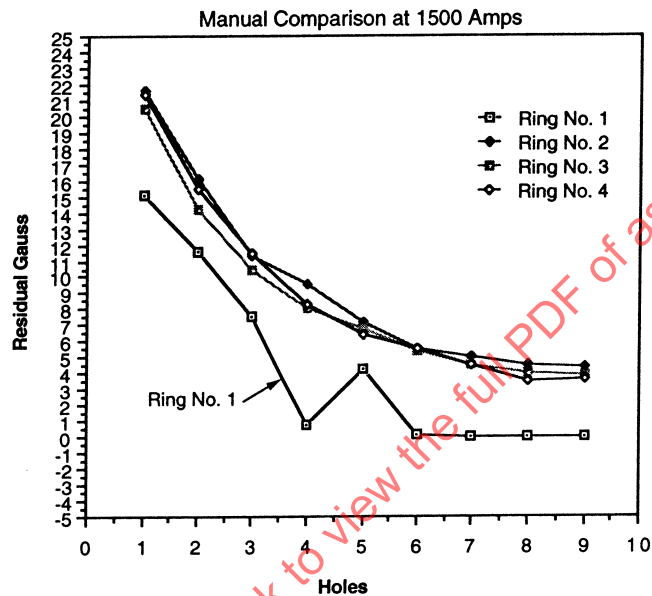
Figure 3 - Flux leakage comparison at 1500 A
