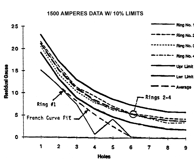
Figure 4 - Residual flux leakage (gauss) results with acceptance criteria
