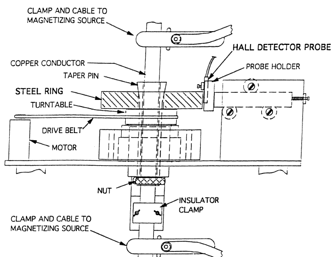
Figure 5 - Steel ring evaluation fixture
