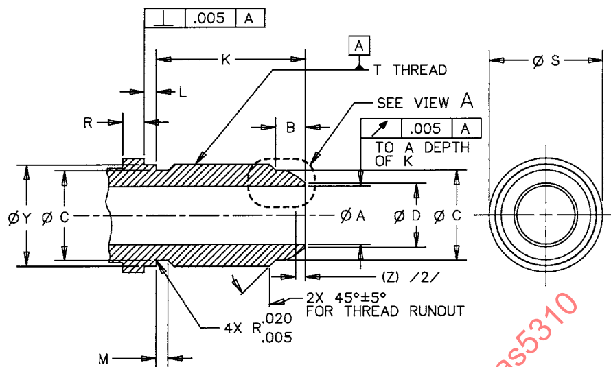
FIGURE 1 - FITTING END, STYLE G
