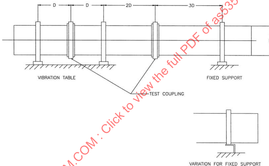
FIGURE 1 - VIBRATION TEST SETUP
