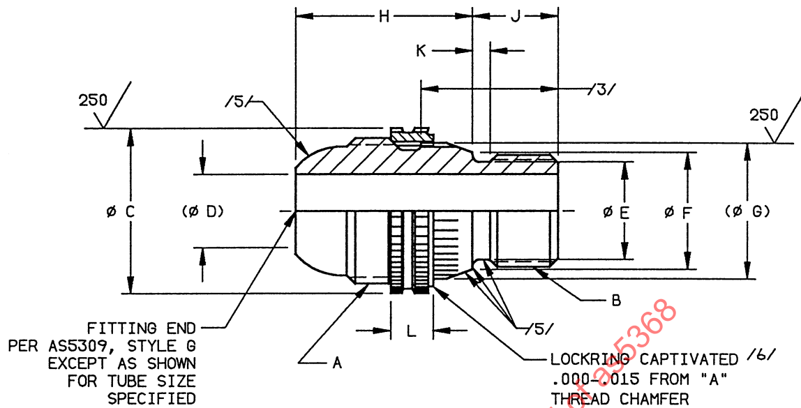
FIGURE 1 - ADAPTER, ASSEMBLY
