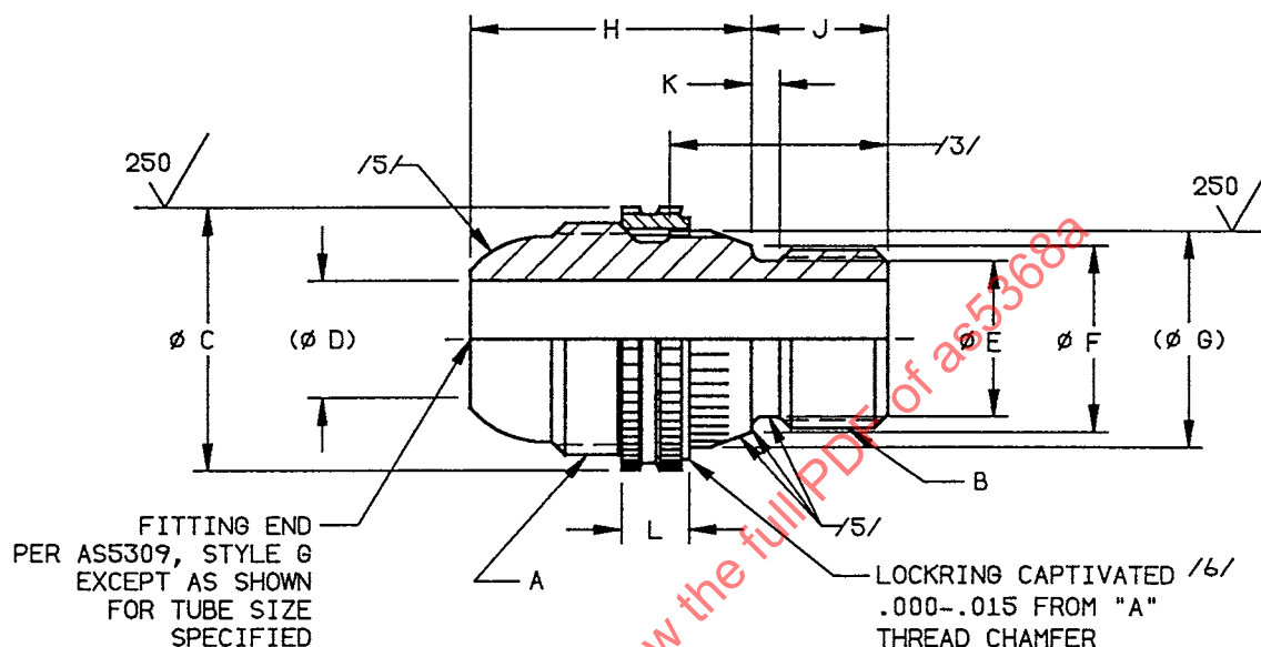
FIGURE 1 - ADAPTER, ASSEMBLY
