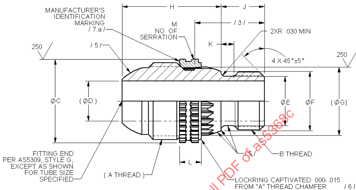
FIGURE 1 - ADAPTER ASSEMBLY
