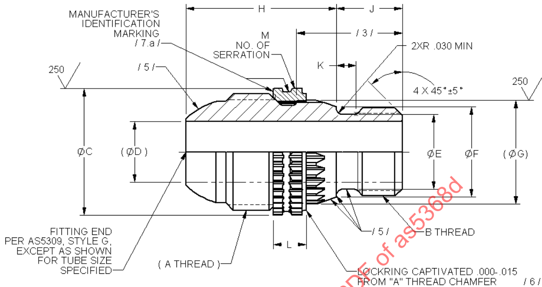
FIGURE 1 - ADAPTER ASSEMBLY
