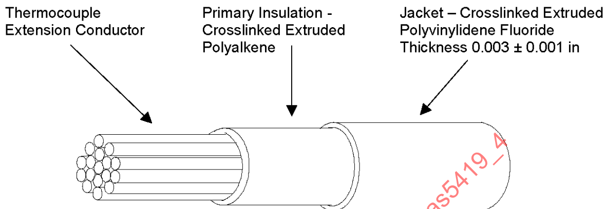
FIGURE 1 - Wire, Thermocouple, Crosslinked Polyalkene Insulated Component wire insulation system must conform to the similar wire type designated in Table 1 of AS5419. Manufacturers must be qualified to AS81044/12 to produce this product.
