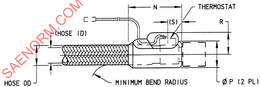
FIGURE 21 - HOSE AND THERMOSTAT DATA
