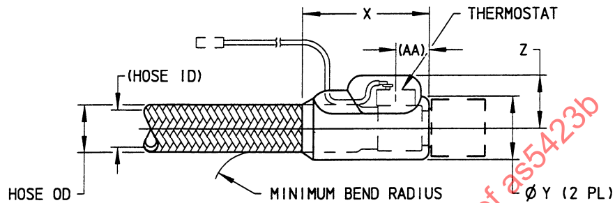
FIGURE 41 - HOSE AND THERMOSTAT DATA
