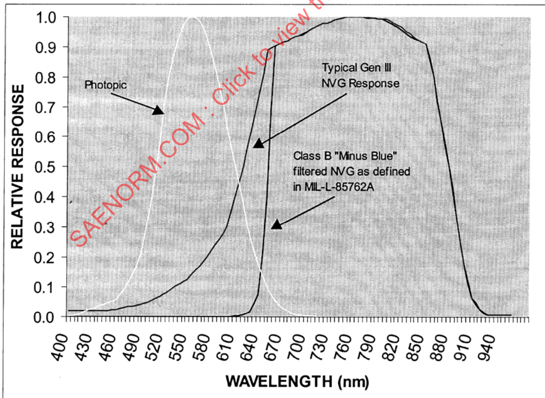
FIGURE 1 - Spectral Response
