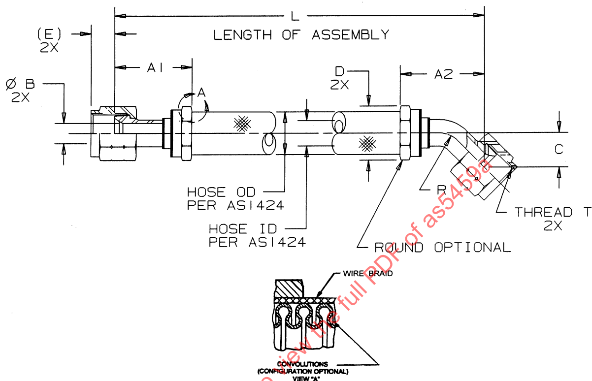
FIGURE 1 - HOSE ASSEMBLY
