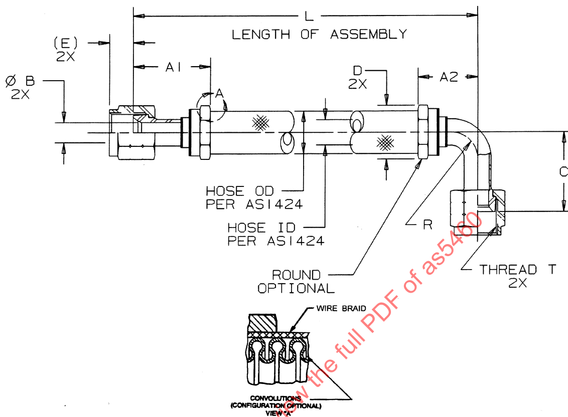
FIGURE 1 HOSE ASSEMBLY
