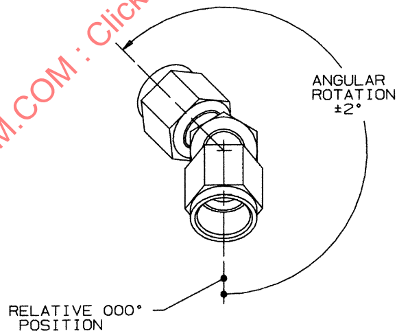
FIGURE 2 - FITTING ANGULAR ORIENTATION /11/
